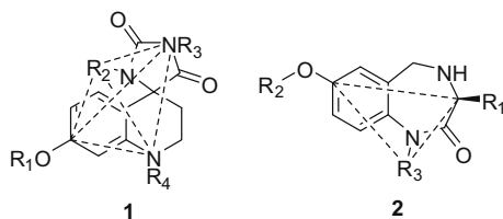
Fig. 1. The \beta -turn mimic scaffold based on the Garland–Dean triangles.
