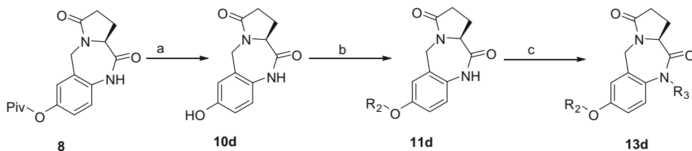
Scheme 3. Solution phase synthetic route of tetrahydro-1,4-benzodiazepine-2-one library. (a) 5% KOH dioxane/H 2 O, 40 min (1:1) (b) R 2 -X, DBU, NMP/DMSO, 4 h, RT (c) i, LiOtBu in THF; ii, R 3 -X in DMSO, 10 h, RT.
