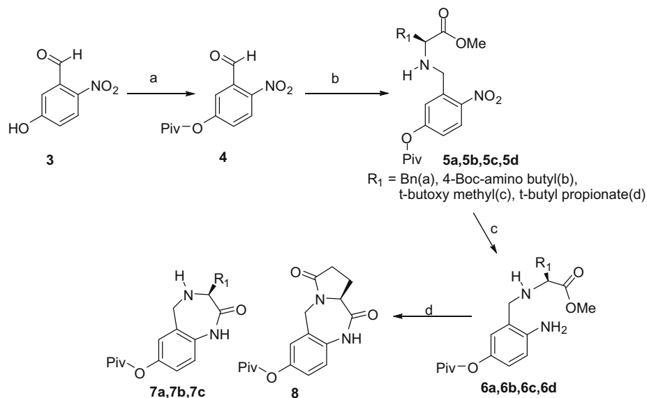
Scheme 1. Preparation of four tetrahydro-1,4-benzodiazepine-2-one scaffolds. (a) trimethylacetyl chloride, TEA, DCM, 30 min RT. (b) Amino acid ester, NaBH(OAc) 3 , DCE/DMF, 2 h, RT. (c) Pd/C, H 2 , MeOH, 3 h, RT. (d) AlMe 3 , toluene, 1 h, 0–25 °C.
